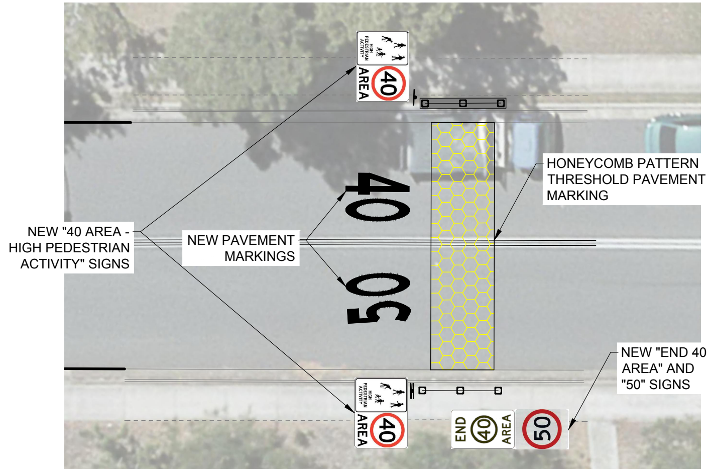
TYPICAL GATEWAY TREATMENT RATIO 1:150
