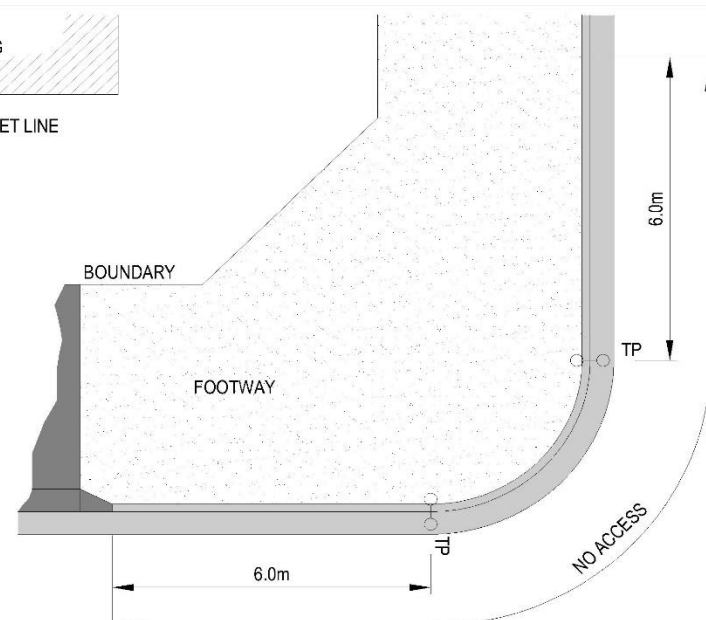
ACCESS RESTRICTION - INTERSECTIONS
