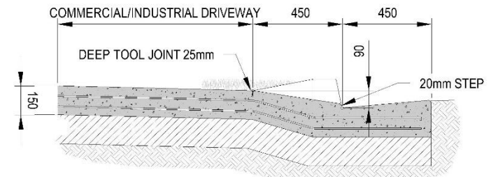
SECTION B-B - UPRIGHT ('SA') KERB COMMERCIAL/INDUSTRIAL
