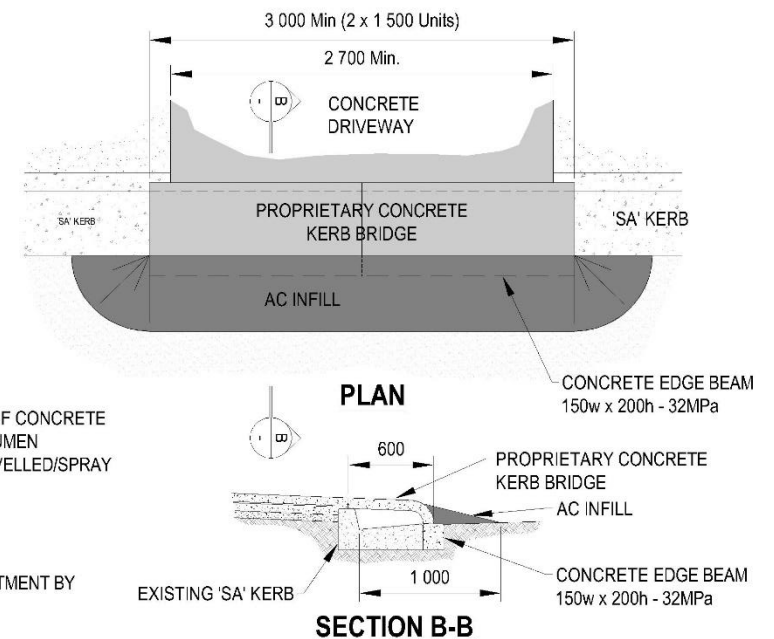
KERB CROSSING FOR UPRIGHT 'SA' KERBS
