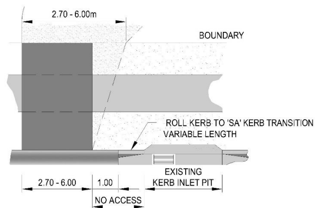
ROLL 'RT' KERB WITH 'SA' KERB INLET
