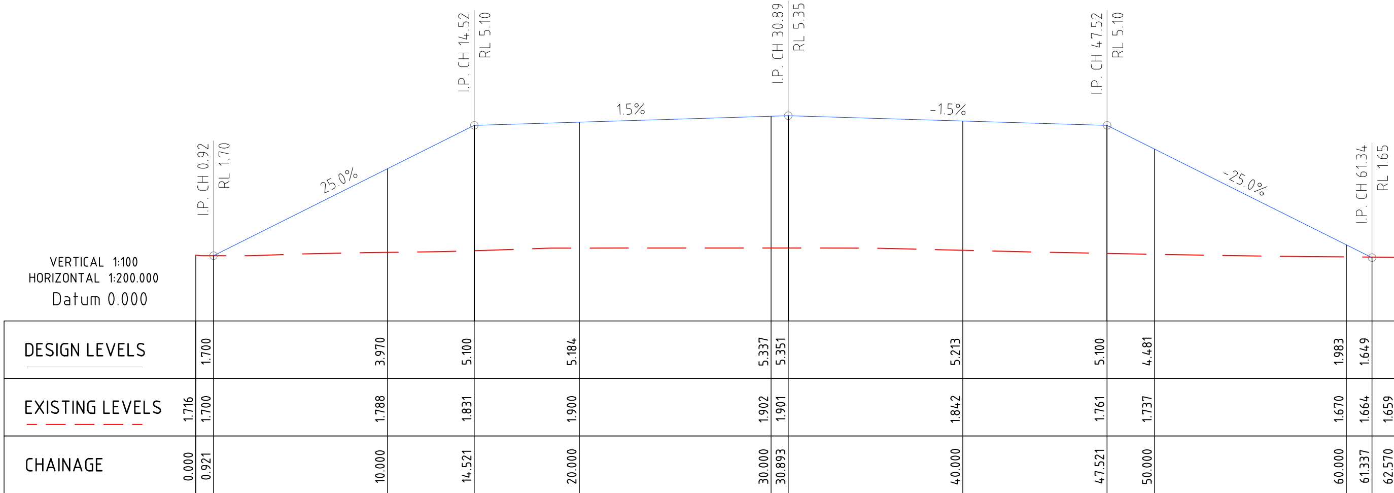
FILL MOUND SECTION C-C
