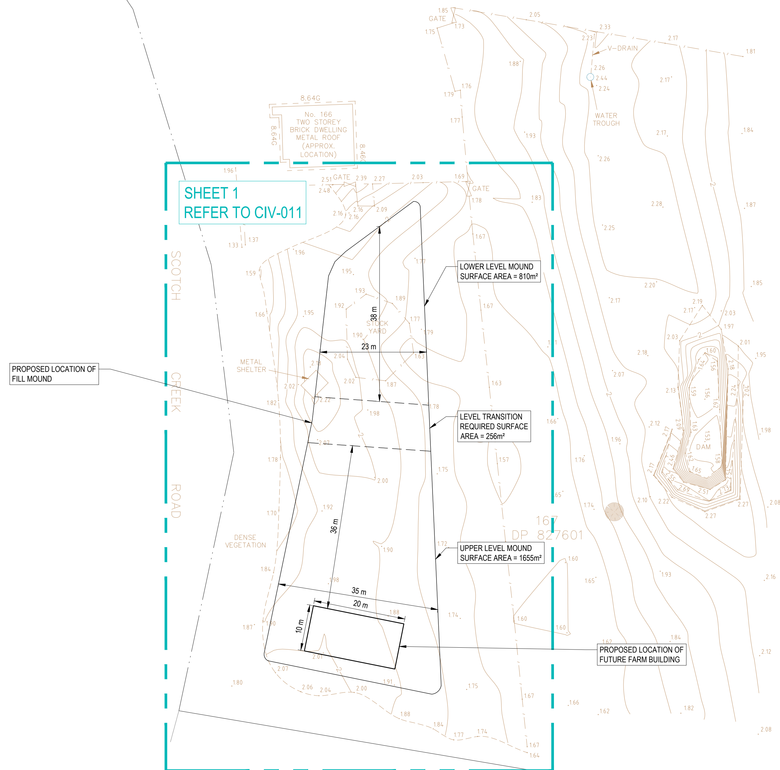
GENERAL ARRANGEMENT PLAN SCALE 1:500
