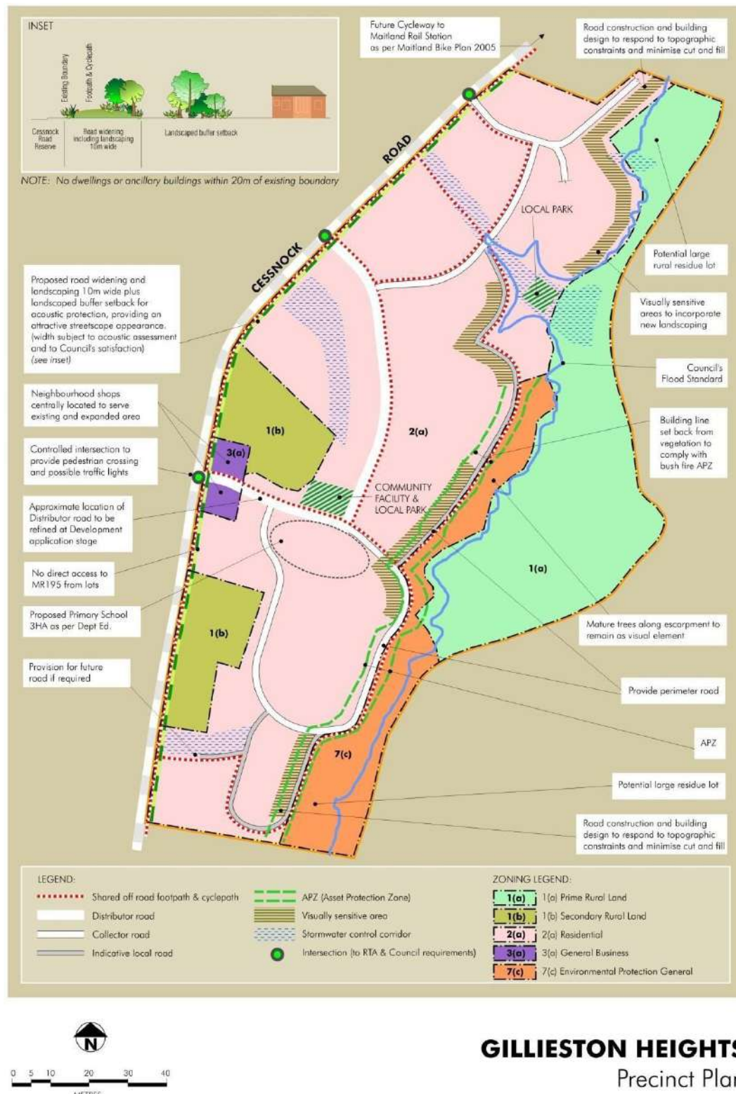
Figure 21: Gillieston Heights East - Precinct Plan
